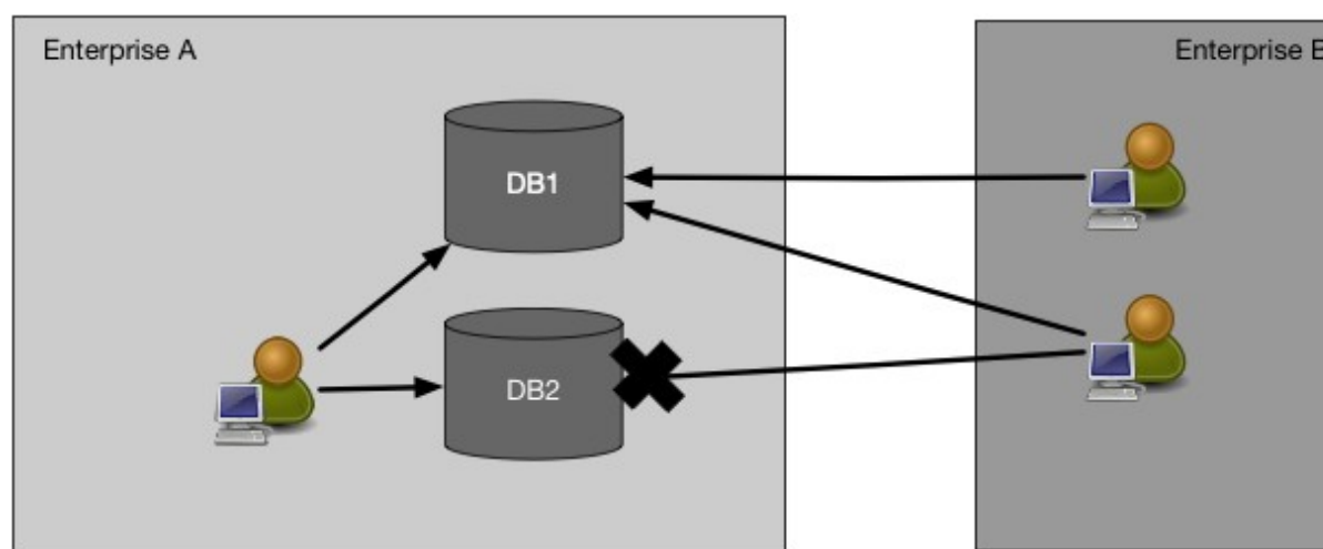
Figure 11: Cross-Enterprise Collaboration
