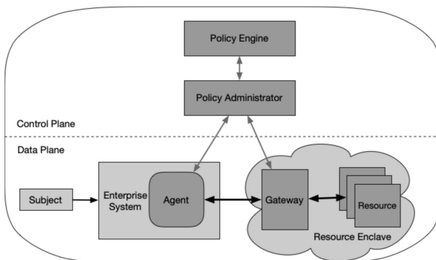
Figure 4: Enclave Gateway Model
