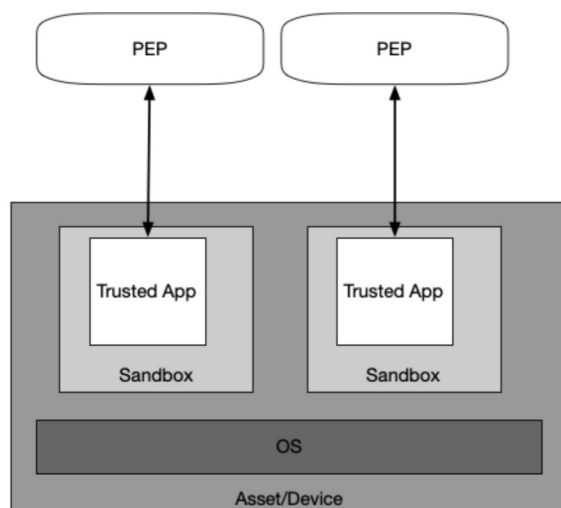
Figure 6: Application Sandboxes
